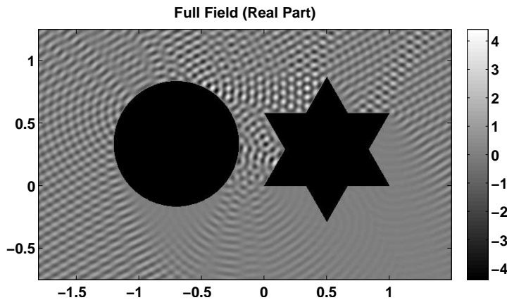
FIG. 8.1. Multiple scattering from a disk and a snowflake domain.
