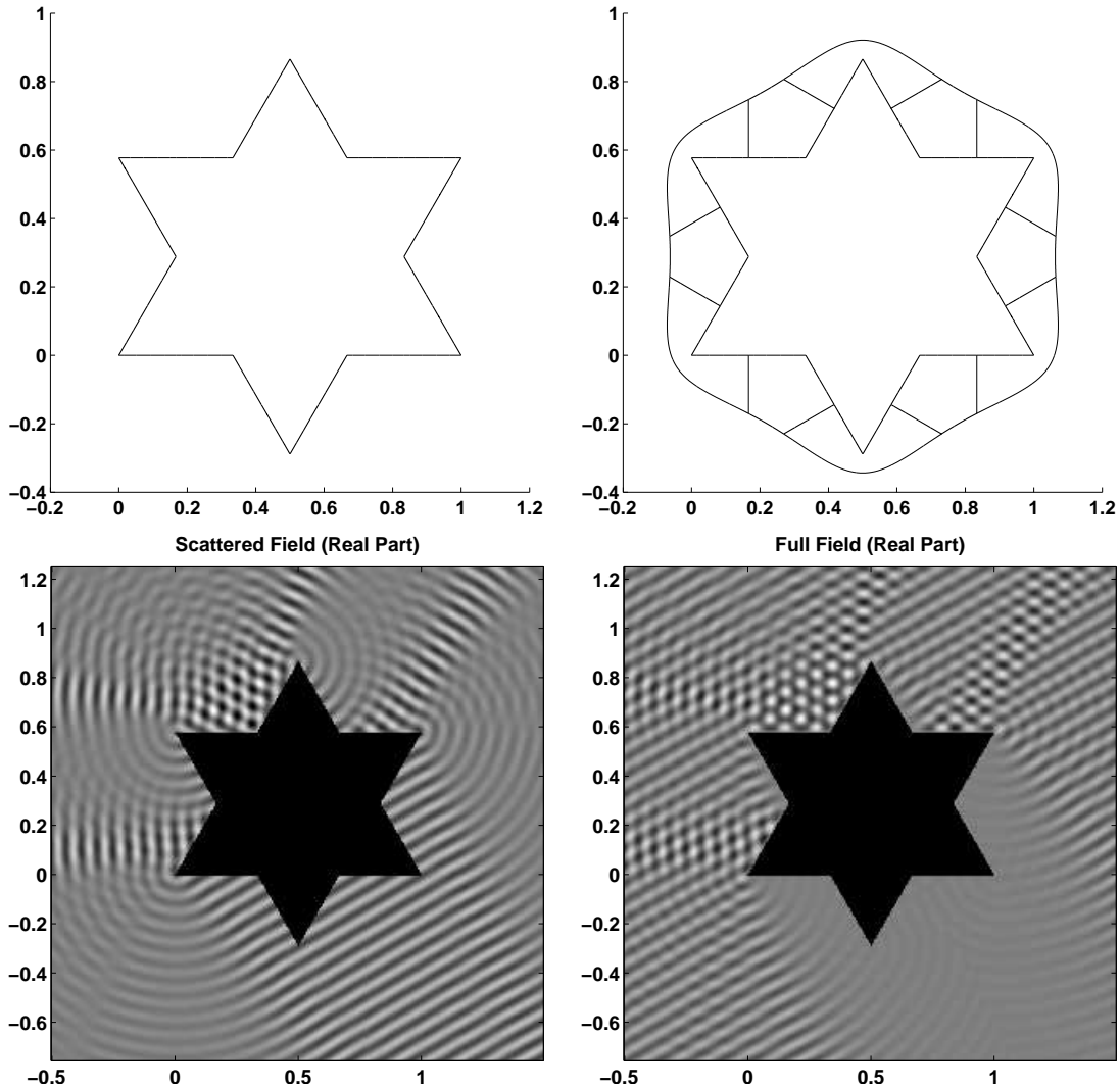
FIG. 6.4. Top plots: A snowflake shaped domain and the corresponding domain decomposition. Bottom plots: The scattered (left) and full field (right) for sound-soft scattering on the snowflake domain.
