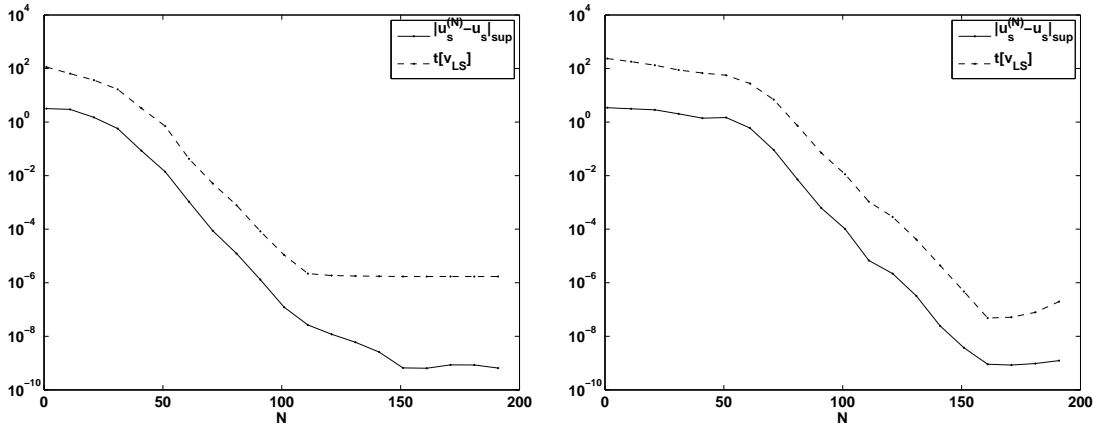
FIG. 6.5. Convergence of t[v_{LS}] (dashed line) for k = 50 (left plot) and k = 100 (right plot). The plots also show an approximation to the convergence of the L^\infty norm of the approximate scattered field u_s^{(N)} in dependence on N to the exact scattered field u_s (solid line).
