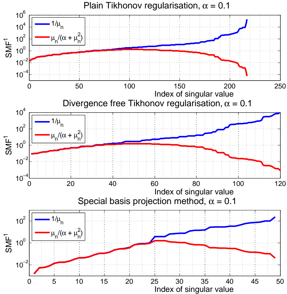
Figure 6. Reciprocal of the singular values of the original matrix and the singular values of the Tikhonov operator with distance of 60 mm between measurement points and resistor network
