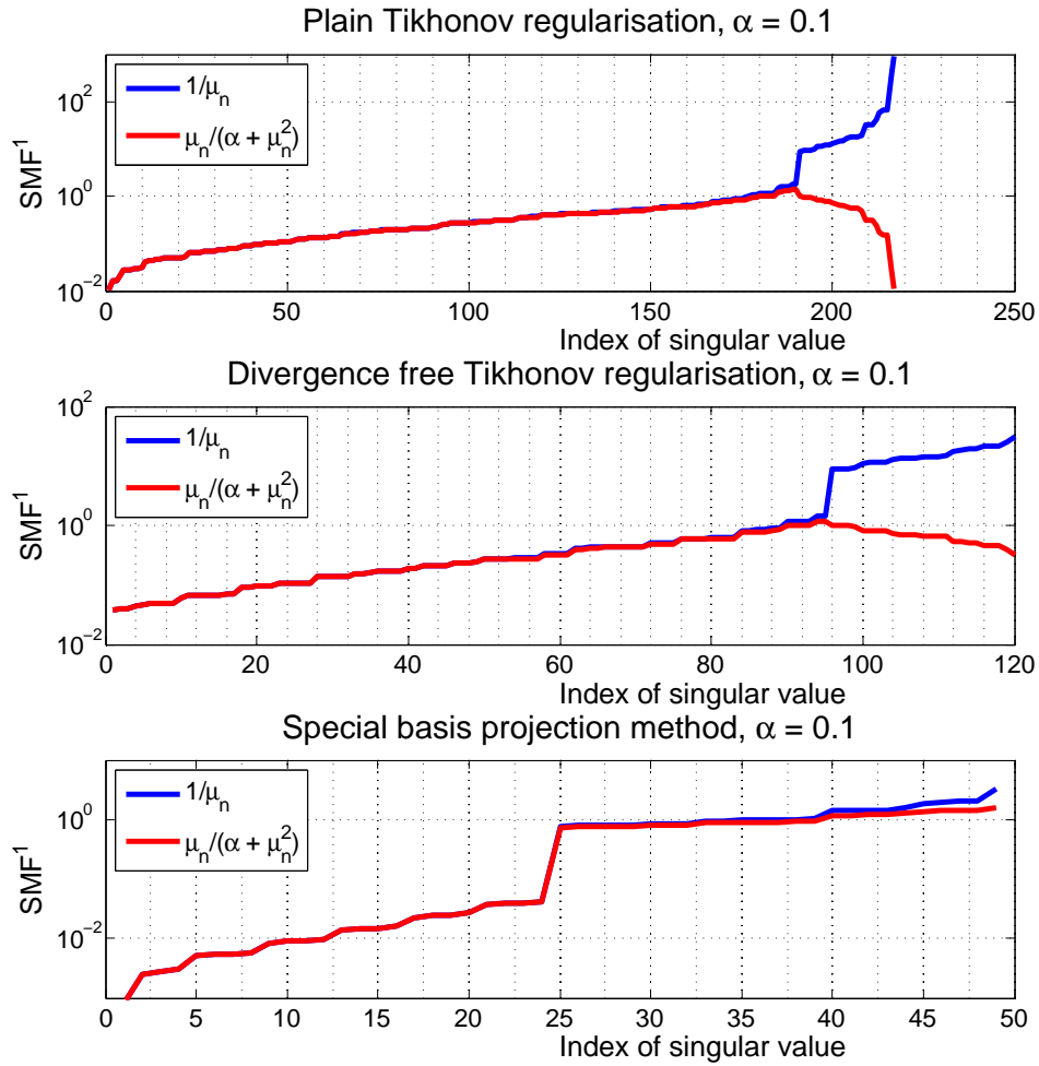
Figure 7. Reciprocal of the singular values of the original matrix and the singular values of the Tikhonov operator with distance of 30 mm between measurement points and resistor network.
